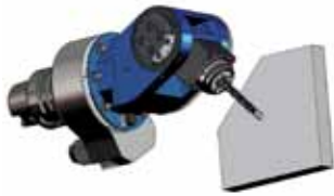
Adjustable angle head 0-100° type FLEX WDX For boring or light duty milling applications at any angle.
